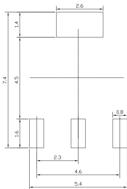
TYPICAL RECOMMENDED STENCIL
