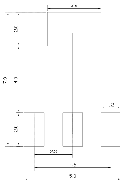
TYPICAL RECOMMENDED LAND PATTERN
