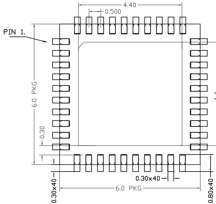
TYPICAL RECOMMENDED LAND PATTERN
